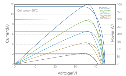
I-V/P-V Curve at Different Temperature (400W)
